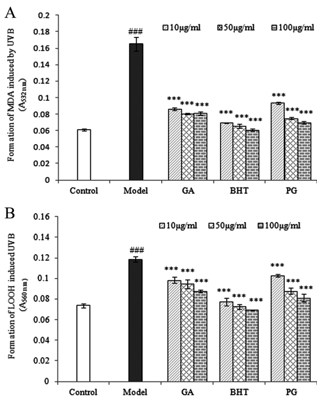
Fig. 2 Effects of TPG on UVB-induced changes in MDA (A) and LOOH (B) levels; data are presented as the mean ± SD (n = 3). TPG, total phenylethanoid glycosides from M. officinalis var. biloba fruits; GA, gallic acid; BHT, butylated hydroxytoluene; MDA, malondialdehyde; LOOH, lipid hydroperoxide. Symbols represent statistical significance. ###p < 0.001, compared with the control group; ***p < 0.001, compared with the model group.
