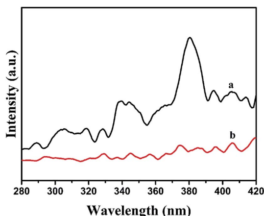
Fig. 6 Photoluminescence spectra of (a) BiOI and (b) \text{BiOI}/\text{Ag}_2\text{CO}_3 (20 wt%).
