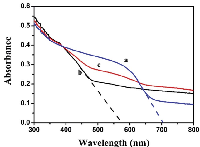
Fig. 5 UV-vis diffuse reflectance spectra of (a) BiOI, (b) \text{Ag}_2\text{CO}_3 and (c) \text{BiOI}/\text{Ag}_2\text{CO}_3 (20 wt%) composite.
