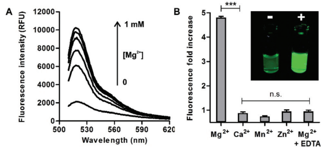
Fig. 2 (A) Fluorescence emission of compound 4 (10 \mu\text{M} , \text{H}_2\text{O} : \text{EtOH} 1 : 1) upon incubation with increasing concentrations (0, 0.1, 0.25, 0.5, 0.75 and 1 mM) of \text{Mg}^{2+} ; \lambda_{\text{exc}} : 450 nm. (B) Comparative fluorescence of compound 4 upon incubation with different divalent cations at their respective physiological concentrations ( \text{Mg}^{2+} , \text{Ca}^{2+} , \text{Mn}^{2+} : 1 mM; \text{Zn}^{2+} : 1 \mu\text{M} ; EDTA: 5 mM). Inset: Pictograms of compound 4 under 365 nm excitation in solutions without (left) or with \text{Mg}^{2+} (right). *** for p < 0.001 , n.s. for p > 0.05 .
