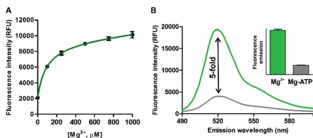
Fig. 3 (A) Determination of the dissociation constant of the \text{Mg}^{2+} - 4 adduct by measuring the fluorescence intensity of compound 4 (10 \mu\text{M} , \text{H}_2\text{O} : \text{EtOH} 1 : 1) at increasing concentrations of \text{Mg}^{2+} . Values represented as means \pm s.e.m. ( n = 3 ). K_d : 92 \pm 30 \mu\text{M} . (B) Emission spectra of compound 4 (50 \mu\text{M} ) upon incubation with 2 mM free \text{Mg}^{2+} (green) and 2 mM \text{Mg} -ATP (grey); \lambda_{\text{exc}} : 450 nm. (Inset) Quantification of the fluorescence intensities for both conditions. Values represented as means \pm s.d. ( n = 3 ).
