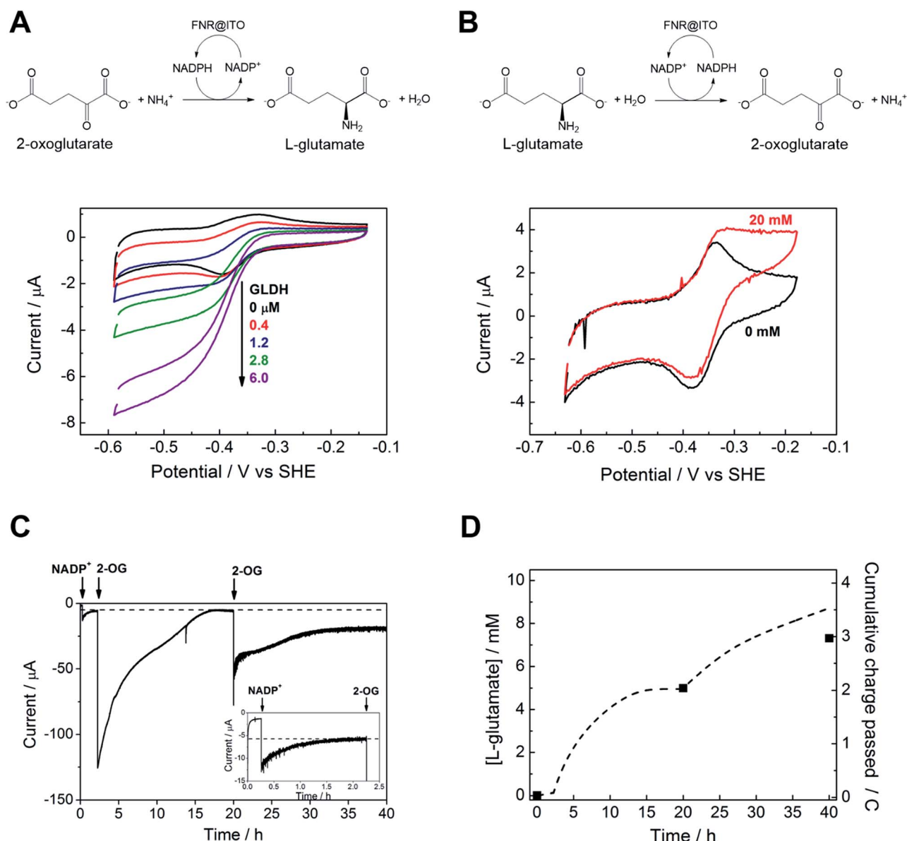
Fig. 4 Coupling FNR@ITO to enzyme-catalysed organic synthesis. (A) Reductive amination of 2-oxoglutarate by glutamate dehydrogenase contained in the cell solution. (NH 4 + 20 mM, 2-oxoglutarate 10 mM, NADP + 50 \mu M, scan rate 5 mV s -1 ). (B) Oxidative deamination of L-glutamate by glutamate dehydrogenase co-loaded on to FNR@ITO electrode (see text for details), NADPH 50 \mu M, L-glutamate 20 mM, scan rate 1 mV s -1 . Other conditions: 25 mM MES, 25 mM TAPS buffer solution at pH 8.0, 20 °C, stationary electrode, solution purged with Ar before measurement. (C) Electrochemical monitoring of L-glutamate synthesis coupled to FNR@ITO. Electrode: FNR@ITO/ITO glass (3 cm 2 ) conditions: electrode potential -0.46 V vs. SHE, 50 mM borate (pH 8.0), cell volume 2.1 mL, NH 4 + 20 mM, glutamate dehydrogenase 4 \mu M, room temperature, constant Ar bubbling. Injections of NADP + 20 \mu M and 2-oxoglutarate 5 mM (twice) are indicated by arrows. Inset shows magnification of the initial 2.5 h. (D) Background-subtracted cumulative charge passed (dashed line) from (C). Black symbols dots refer to direct measurement of L-glutamate concentration by NMR spectroscopy.
