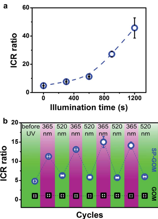
Fig. 4 Time evolution and reversibility. (a) The rectification ratio of the SP-GOM gradually enhances with prolonged illumination time. (b) Repeated cycles under alternating UV and visible light irradiation. The SP-GOMs show excellent reversibility in the ionic rectifying properties controlled by light. In contrast, the unmodified GOMs are insensitive to light irradiation showing non-rectified ion transport behavior. The concentration of SP for chemical modification is 0.6 \text{ mg ml}^{-1} .
