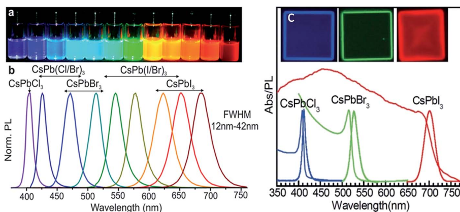
Fig. 9 (a) Colloidal perovskite \text{CsPbX}_3 NCs ( X = \text{Cl}, \text{Br}, \text{I} ) solutions in toluene under a UV lamp ( \lambda = 365 nm); (b) representative PL spectra ( \lambda_{\text{exc}} = 400 nm for all but 350 nm for \text{CsPbCl}_3 nanocrystals). (c) Optical absorption and PL spectra of \text{CsPbCl}_3 , \text{CsPbBr}_3 , and \text{CsPbI}_3 nanoplatelets. Inset: PL image of \text{CsPbCl}_3 , \text{CsPbBr}_3 , and \text{CsPbI}_3 nanoplatelets. Reprinted with permission from ref. 40 and 49, copyright 2015, American Chemical Society and 2016, Advanced Material.
