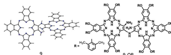
Scheme 2 Schematic of the molecular structures of the relatively stable di-tribenzotetrazaporphyrinato-amine intermediates 9 and (9-OR).
