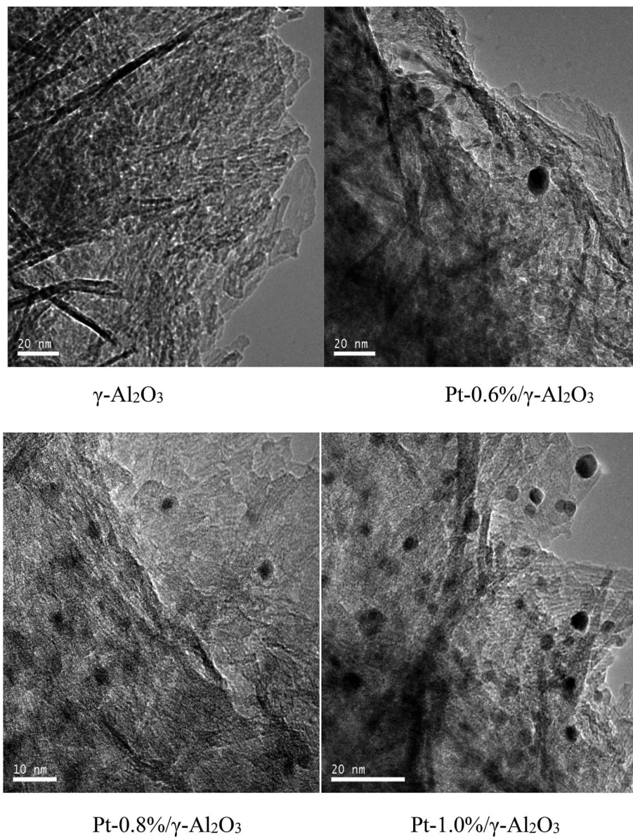
Fig. 1 TEM micrographs of the \gamma\text{-Al}_2\text{O}_3 carrier and the \text{Pt}/\gamma\text{-Al}_2\text{O}_3 catalyst.
