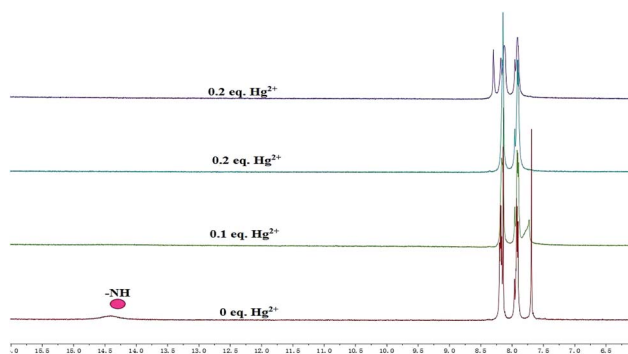
Fig. 7 Partial ^1\text{H} NMR spectra of Z-3 in DMSO- d_6 with different concentrations of \text{Hg}^{2+} .
