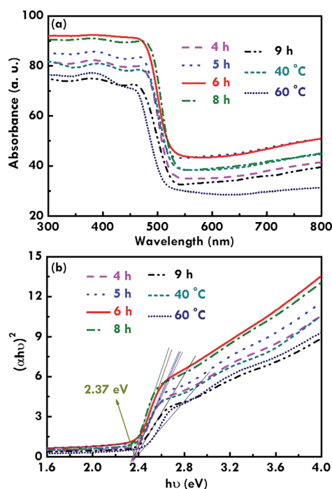
Fig. 5 (a) Absorption spectra and (b) Tauc plots for BiVO 4 electrodes synthesized using a reaction time of 4 h at 40 °C and 4 h at 60 °C (4 h), 5 h at 40 °C and 5 h at 60 °C (5 h), 6 h at 40 °C and 6 h at 60 °C (6 h), 8 h at 40 °C and 8 h at 60 °C (8 h), 9 h at 40 °C and 9 h at 60 °C (9 h), 12 h at 40 °C (40 °C), and 12 h at 60 °C (60 °C).
