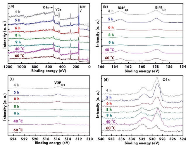
Fig. 4 The XPS spectra of the BiVO 4 prepared using different reaction times and temperatures. (a) The survey XPS spectrum, (b) Bi 4f, (c) V 2p, and (d) O 1s peaks related to the BiVO 4 photocatalyst.
