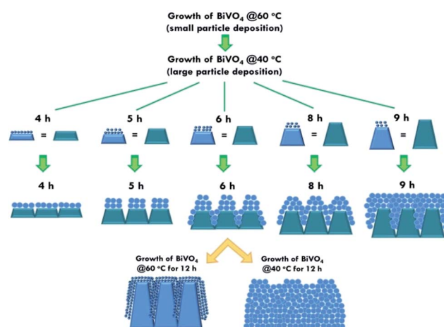
Fig. 2 The scheme for illustrating the growth of BiVO 4 prepared in different conditions. The cartons in the top side present the growth of the BiVO 4 nanostructures in two steps. The reaction temperatures for the first and second steps are 60 and 40 °C, respectively. The cartons in the bottom side present the growth of the BiVO 4 nanostructures in the one step with a reaction time of 12 h, and the reaction temperature was kept at 40 or 60 °C for the whole reaction process.
