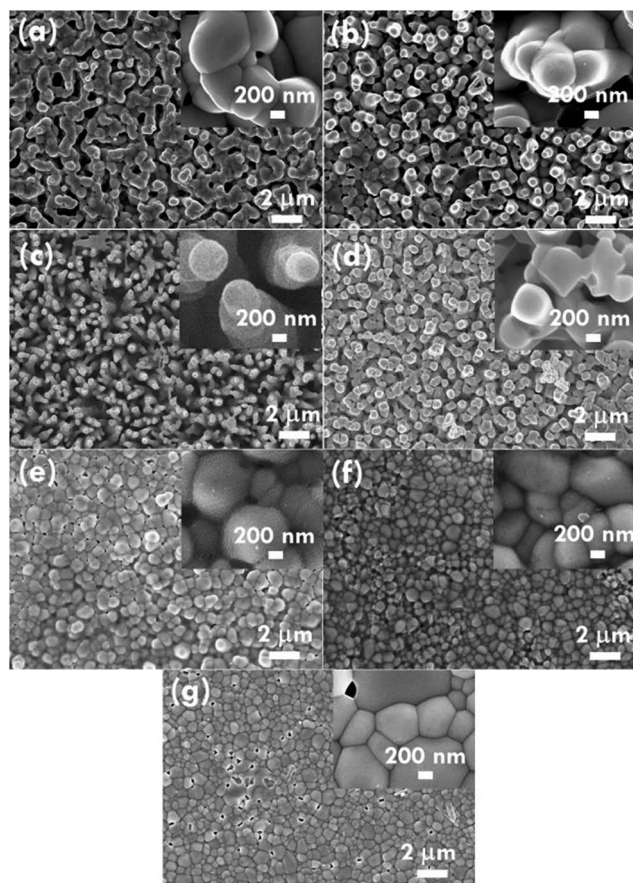
Fig. 1 The SEM images for the BiVO 4 electrode synthesized using reaction times of (a) 4 h, (b) 5 h, (c) 6 h, (d) 8 h, and (e) 9 h for the first and second step of the refluxing process and 12 h for the one step refluxing process with the reaction temperature of (f) 40 °C and (g) 60 °C.
