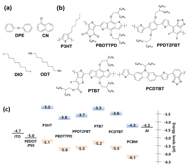
Fig. 1 The molecular structure of the (a) processing additives and (b) donor polymers. (c) The energy band diagram of the components in the PSCs.
