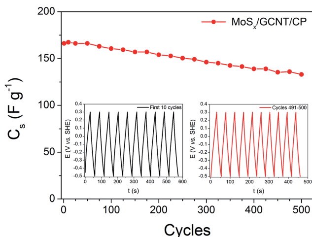
Fig. 7 Degradation test of the \text{MoS}_x/\text{GCNT}/\text{CP} electrode performed with 500 charge/discharge cycles at 5 \, \text{A} \, \text{g}^{-1} , showing the degradation of electrode specific capacitance during the test, with (insets) plots of the first and last 10 charge/discharge cycles (time axes t are referenced to the beginning of each 10-cycle set).
