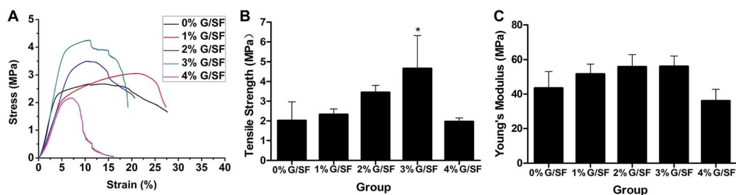
Fig. 8 Mechanical properties of G/SF fibrous scaffolds: (A) stress–strain curves, (B) tensile strength, and (C) Young's modulus. *Indicates significant difference of p < 0.05 .
