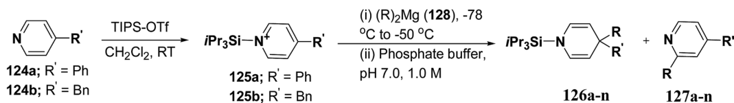
Scheme 39 Synthesis of 1,4-DHPs 126a–n via addition reaction of Grignard reagent to N -triisopropylsilylpyridinium ions 125a–b.
