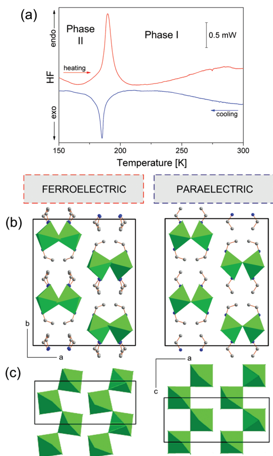
Fig. 1 (a) DSC data confirming the transition sequence seen in ECB (rate: 10 K min^{-1} , sample mass: 12.86 mg); (b) the structure overview of the paraelectric Phase I (right) and ferroelectric Phase II (left); (c) [BiCl_5]^{2-}_\infty chains propagate along the c -direction and distinctly deform after the PT.
