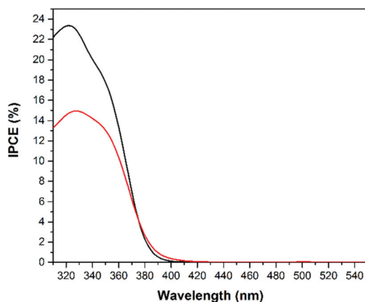
Fig. 8 IPCE spectra for water oxidation measured for cold sprayed \text{TiO}_2 on titanium metal (red) and screen printed \text{TiO}_2 on FTO (black) photoanodes. Measurements for water oxidation were conducted in an aqueous 0.5 M \text{H}_2\text{SO}_4 solution at a bias of 1 V vs. NHE.
