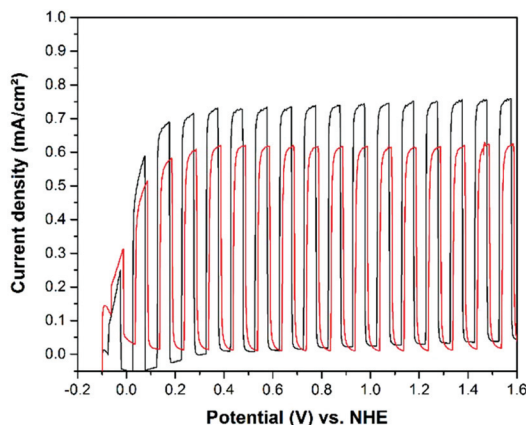
Fig. 7 Chopped light current–potential curves of cold sprayed \text{TiO}_2 on titanium metal (red) and screen printed \text{TiO}_2 on FTO (black) photoanodes in 0.5 M \text{H}_2\text{SO}_4 with addition of 10 vol% of methanol ( \sim 2 \text{ mol L}^{-1} ). Measured with a scan rate of 20 \text{ mV s}^{-1} . Current densities were measured upon irradiation with AM 1.5-global light (300 W Xe lamp).
