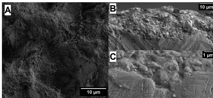
Fig. 4 (A) SEM surface morphology image of a cold sprayed \text{TiO}_2 film. (B) Cross-sectional SEM image of a cold sprayed \text{WO}_3 film on a titanium substrate at a magnification of 1400 \times . (C) Cross-sectional SEM image of the interface between the cold sprayed \text{WO}_3 film and the titanium substrate at a magnification of 8500 \times .
