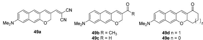
Fig. 28 Structures of the fluorescent chemosensors 49a–e .
