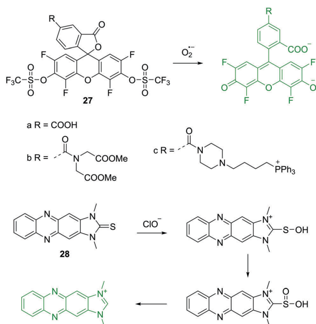
Fig. 13 Structures and proposed mechanism of 27 and 28 for detection of \text{O}_2^{\cdot-} and \text{ClO}^- respectively.
