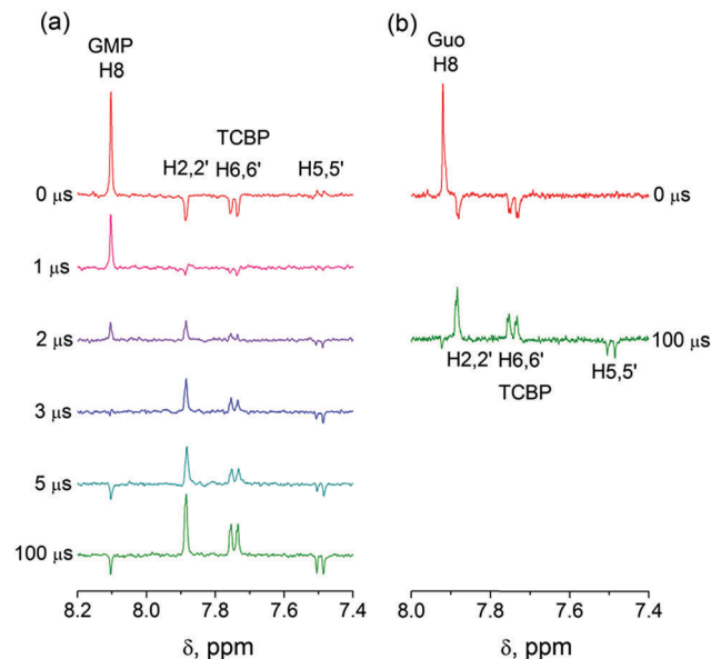
Fig. 1 (a) 1 H CIDNP spectra, detected in the photoreaction of 2 mM 3,3',4,4'-tercarboxy benzophenone and 20 mM guanosine-5'-monophosphate in 50 mM sodium phosphate buffer at pH 6.9 at variable time delays after the laser pulse. The delays are ascending from 0 (top) to 100 μs (bottom spectrum). (b) 1 H CIDNP spectra detected in the photoreaction of 2 mM 3,3',4,4'-tercarboxy benzophenone and 2 mM guanosine in 50 mM sodium phosphate buffer at pH 6.9. The upper spectrum was taken immediately after the laser pulse, and the lower spectrum at 100 μs after the laser pulse.
