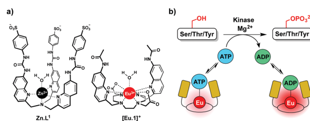
Fig. 1 (a) Structures of complexes \text{Zn} \cdot \mathbf{L}^1 and [\text{Eu} \cdot \mathbf{1}]^+ ; (b) cartoon illustrating continuous monitoring of kinase activity using [\text{Eu} \cdot \mathbf{1}]^+ . The \text{Eu}(\text{III}) complex binds reversibly to ATP and ADP, providing a ratiometric luminescent signal that precisely indicates the ADP/ATP ratio.
