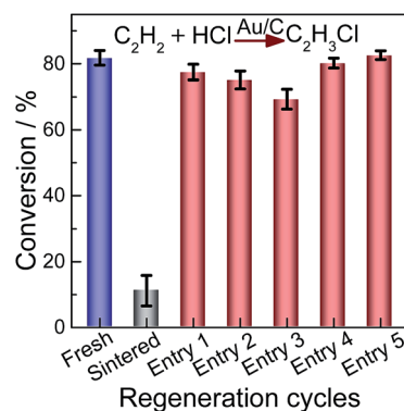
Fig. 7 Relative catalytic activity of acetylene hydrochlorination over the fresh, sintered and regenerated Au/C catalysts. Entries 1–3: sintered Au/C regenerated directly with CHI_3 at 40 \text{ }^\circ\text{C} ; Entries 4 and 5: sintered Au/C catalyst regenerated with CHI_3 containing HAuCl_4 (0.002 M) at 40 \text{ }^\circ\text{C} .
