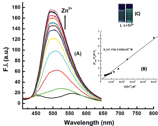
Fig. 4 (A) Fluorescence titration of H_3SAL-NH ( 20 \mu M ) in HEPES buffer at pH 7.2 recorded in THF : H_2O (6 : 4, v/v) with the gradual addition Zn(NO_3)_2 \cdot 6H_2O with \lambda_{ex} = 398 nm and \lambda_{em} = 498 nm. (B) B–H plot of F.I. vs. 1/[Zn^{2+}] ; (C) UV-exposed emission image of H_3SAL-NH with Zn^{2+} .
