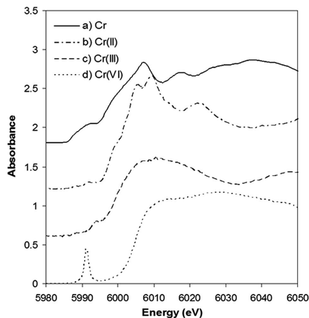
Fig. 4 Normalized Cr K-edge XANES spectra of (a) Cr(0) metal, (b) Cr(II) acetate, (c) \text{Cr}_2\text{O}_3 , and (d) \text{CrO}_3 . These spectra have been vertically shifted for clarity
