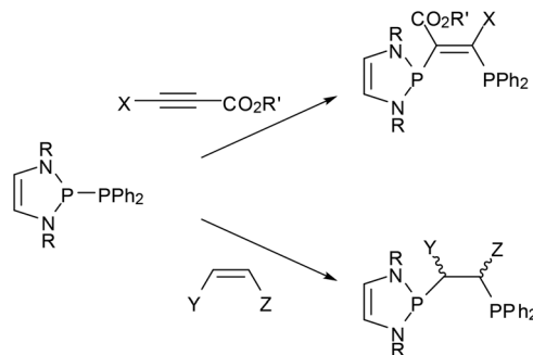
Scheme 8 Addition of P-phosphino-DAPs (R = tBu, Mes, CH(Cy)Me) to activated alkynes (R' = Me, Et; X = H, CO 2 R') and alkenes (Y = CO 2 Me, H; Z = CO 2 Me, H; Y = CN, Z = H).
