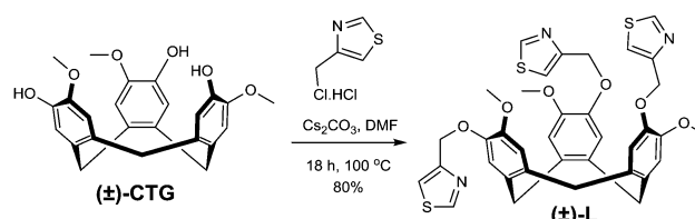
Scheme 1 Synthetic route to (±)-tris-(4-methylthiazolyl)cyclotruguaiacylene.
