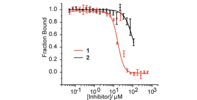
Fig. 3 Biophysical screening of helix mimetic 1 and hybrid 2 to profile selectivity; FA competition data for inhibition of p53/hDM2.
