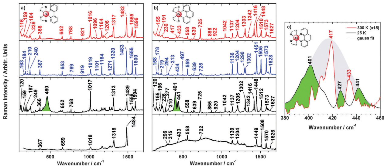
Fig. 11 Temperature dependence of the resonance Raman ( \lambda_{\text{exc}} = 647 \text{ nm} ) spectra of 1 (a) and 2 (b) at 300 K (red lines), 100 K (blue lines) and 25 K (black lines) in KBr-pellet and vacuum deposited film ( \lambda_{\text{exc}} = 514 \text{ nm} ) on Au/Ti/glass at 25 K (black lines, bottom). Resonance Raman ( \lambda_{\text{exc}} = 647 \text{ nm} ) of 2 (c) in KBr at 300 K (red line, 15 \times enlarged), 25 K (black line) and the Gaussian profile of the 25 K spectrum (grey area). The electronic Raman transition bands are coloured in green.
