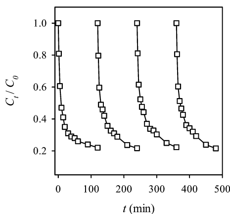
Fig. 13 Recyclability of MIL-88A to activate persulfate for the RB decolorization (persulfate = 200 mg L -1 , MIL-88A = 500 mg L -1 , 40 °C).
