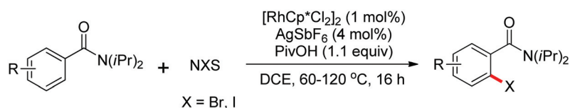
Scheme 93 [Rh(III)Cp*]-catalyzed ortho -bromination and iodination of arenes.
