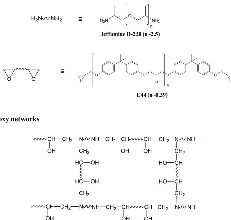
Fig. 1 Chemical structures of the epoxy precursors and cured networks.
