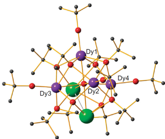
Fig. 4 Structure of [(\text{Dy})_4\text{K}_2\text{O}(\text{OtBu})_{12}] with hydrogen atoms omitted for clarity. Reprinted by permission from Macmillan Publishers Ltd, ref. 8, copyright 2013.
