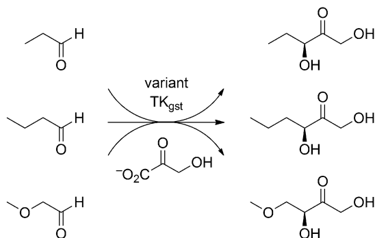
Scheme 1 Carboligation reactions studied for directed evolution of TK gst towards increased activity and stereoselectivity with generic aldehydes.
