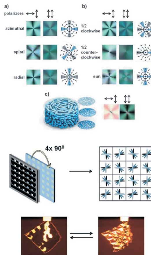
Fig. 4 (a) Examples of crosslinked LC polymer films with circular alignment patterns as viewed between crossed or parallel polarizers. Bottom: illustration of circular twisted nematic alignment and images of the resulting film between perpendicular and parallel polarizers. Reproduced with permission from ref. 84. Copyright 2012, Wiley-VCH. (b) The deformation of crosslinked LC polymer films with checkerboard alignment pattern upon photothermal heating with IR light of a film with a checkerboard pattern. Reproduced with permission from ref. 85. Copyright 2013, Wiley-VCH.
