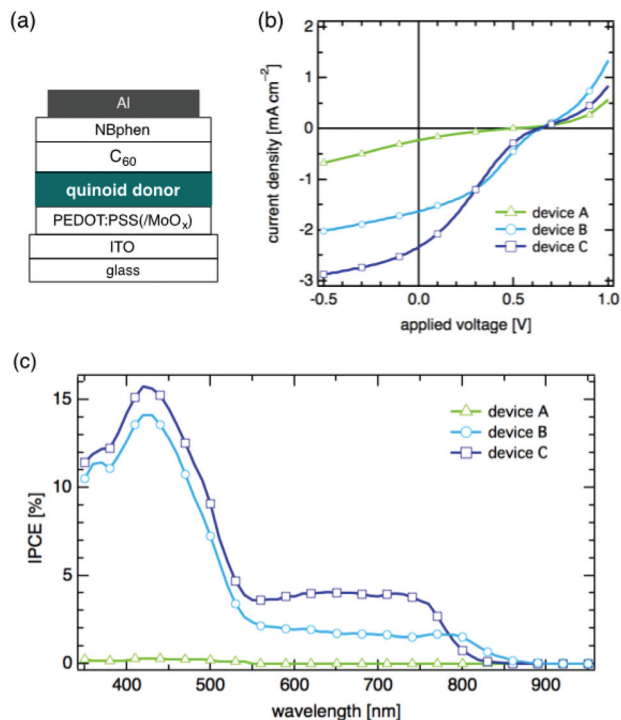
Fig. 3 The configuration of the fabricated OSC devices A, B, and C using the quinoid materials 1, 2, and 3, respectively, as a donor layer (a), J–V characteristics (b) and IPCE profiles (c) of the devices. For devices B and C, a molybdenum oxide ( \text{MoO}_x ) layer was inserted between the PEDOT:PSS and the quinoid donor layers.
