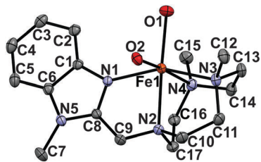
Fig. 1 Molecular structure of [Fe II (H 2 O) 2 (Me 2 ,BzIm-TACN)] 2+ (1 H 2 O ) with 30% probability ellipsoids; H-atoms have been omitted for clarity.
