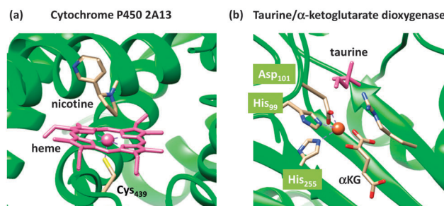
Fig. 1 Active site structures of two typical mononuclear iron enzymes: (a) cytochrome P450 from 4EJG pdb file and (b) taurine/ \alpha -ketoglutarate dioxygenase from 1O57 pdb file.
