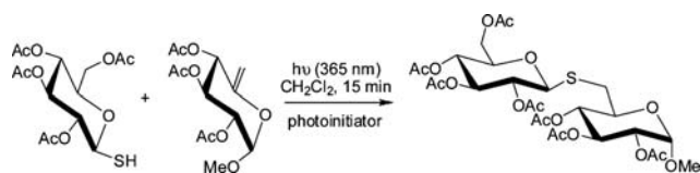
Scheme 32 Radical-induced thiol-ene coupling between a peracetylated glucosylthiol and a hex-5-ene-pyranoside under photochemical conditions.
