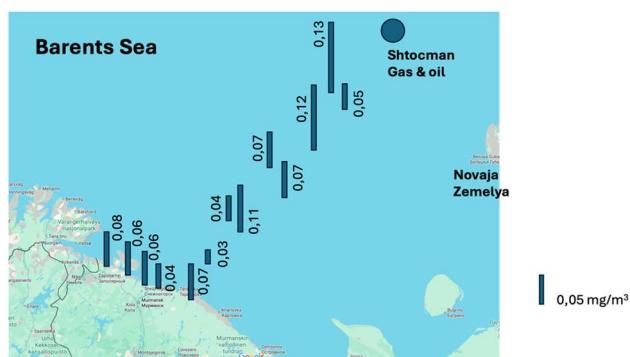
Fig. 18 Distribution of petroleum hydrocarbons in the surface waters [ \text{mg m}^{-3} ] along the projected Shtocman pipeline. Report IMR/PINRO; Joint report Barents Sea 2007.
