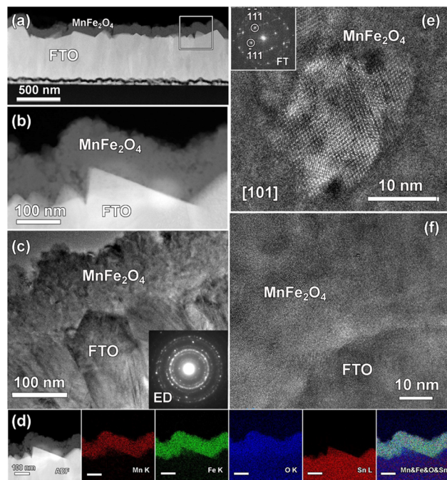
Fig. 7 (a) Cross-sectional low magnification HAADF-STEM image of a sample obtained from a Mn:Fe = 1:2 precursor mixture. (b) Magnified image of the region framed by the white box in (a). (c) BF-TEM image of MnFe 2 O 4 /FTO interface and corresponding ring ED pattern. (d) HAADF-STEM image and simultaneously acquired EDXS elemental maps for Mn K, Fe K, O K, and Sn L signals, together with an overlaid color image. (e) High resolution HAADF-STEM image of an individual MnFe 2 O 4 nanoparticle recorded along the [101] zone axis, and corresponding FT pattern. (f) High resolution HAADF-STEM image of MnFe 2 O 4 /FTO interface.
