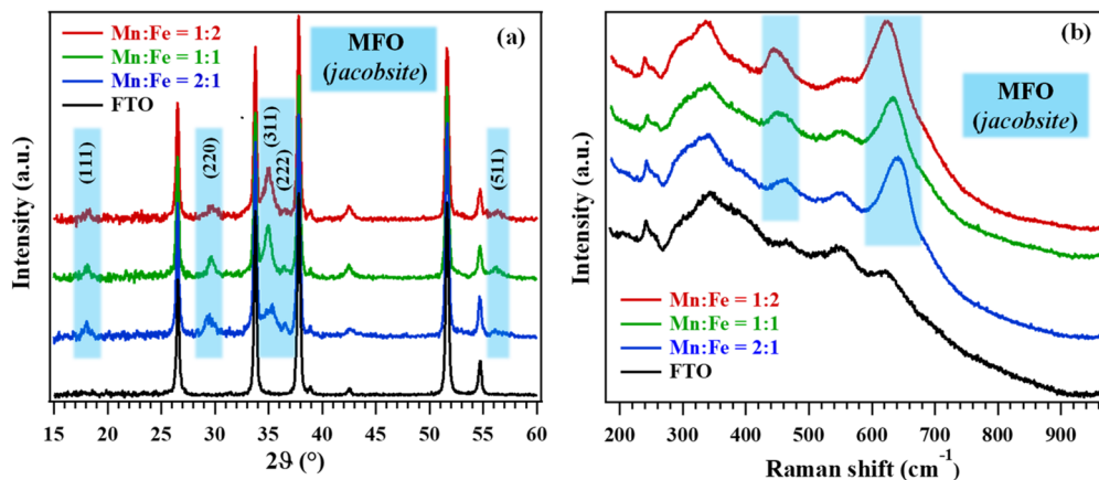
Fig. 2 (a) XRD patterns and (b) Raman spectra for MFO specimens grown on FTO from different mixtures of \text{Mn}(\text{hfa})_2\cdot\text{TMEDA} and \text{Fe}(\text{hfa})_2\cdot\text{TMEDA} precursors. Curves have been vertically shifted for clarity. The XRD pattern and Raman spectrum of the bare FTO substrate are also reported for comparison. In both panels, the main signals from the MFO spinel phase are highlighted by a pale blue background.
