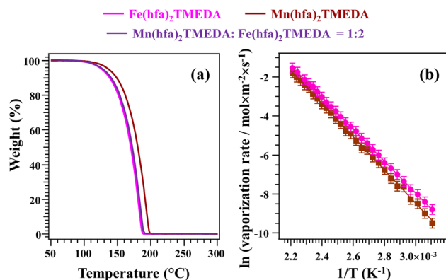
Fig. 1 (a) TGA curves in \text{N}_2 for \text{Mn(hfa)}_2\text{TMEDA} (brown), \text{Fe(hfa)}_2\text{TMEDA} (pink) and their 1 : 2 mixture (violet). (b) Arrhenius plots for the vaporization of the two precursors (temperature interval \approx 50 \div 180^\circ\text{C} ).
