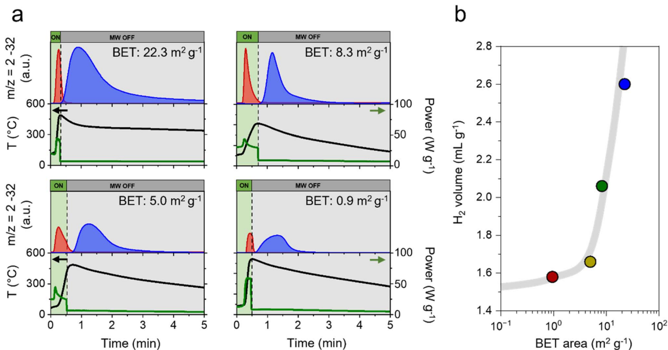
Fig. 6 Surface area amplifies hydrogen production in Ce 0.9 La 0.1 O 1.95 . (a) H 2 and O 2 evolution profiles during microwave-driven water splitting cycles for samples with varying surface areas (samples sintered at 700, 900, 1200, and 1400 °C); (b) variation of the amount of H 2 produced with respect to the BET area.
