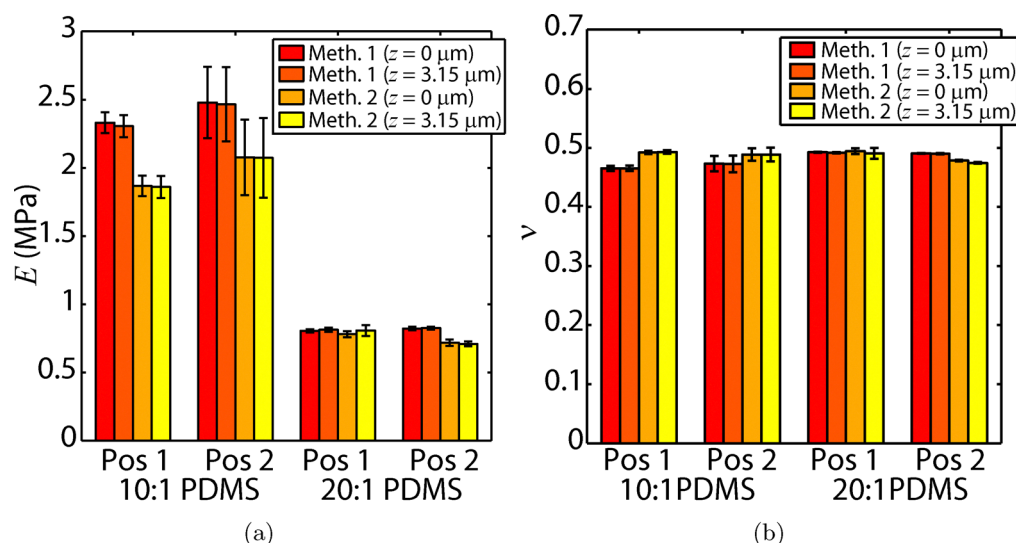
Fig. 9 Comparison of (a) E and (b) \nu calculated from the PT method (Method 1) and the hybrid method (Method 2) using displacements calculated from the FE model along the specimen surface and 3.15 \mu\text{m} below the surface assuming perfectly bonded contact between the indenter and film. The height of each bar represents the corresponding mean, and each error bar represents the corresponding standard deviation.
