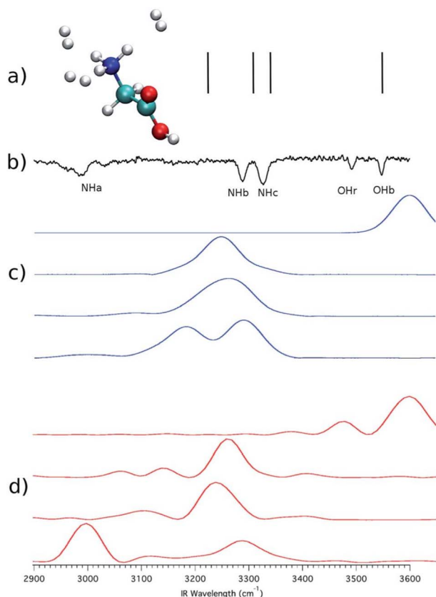
Fig. 2 Vibrational spectra of protonated glycine microsolated by three \text{H}_2 molecules. Panel (a): scaled harmonic estimates; panel (b): experimental spectrum; panel (c): QCT method results; panel (d): DC-SCIVR calculation. Reproduced from F. Gabas, G. Di Liberto, R. Conte and M. Ceotto, Chem. Sci. , 2018, 9, 7894–7901.
