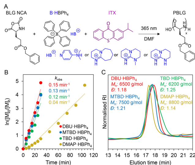
Fig. 2 Schematic of synthetic route for polypeptides using different PBGs, (B) kinetic plot of \ln([M]_0/[M]_t) versus time for BLG NCA photo-ROP with different PBGs ([M] = 0.4 M, [M] 0 /[I] 0 = 50) in DMF, and (C) normalized SEC traces of corresponding polypeptides.
