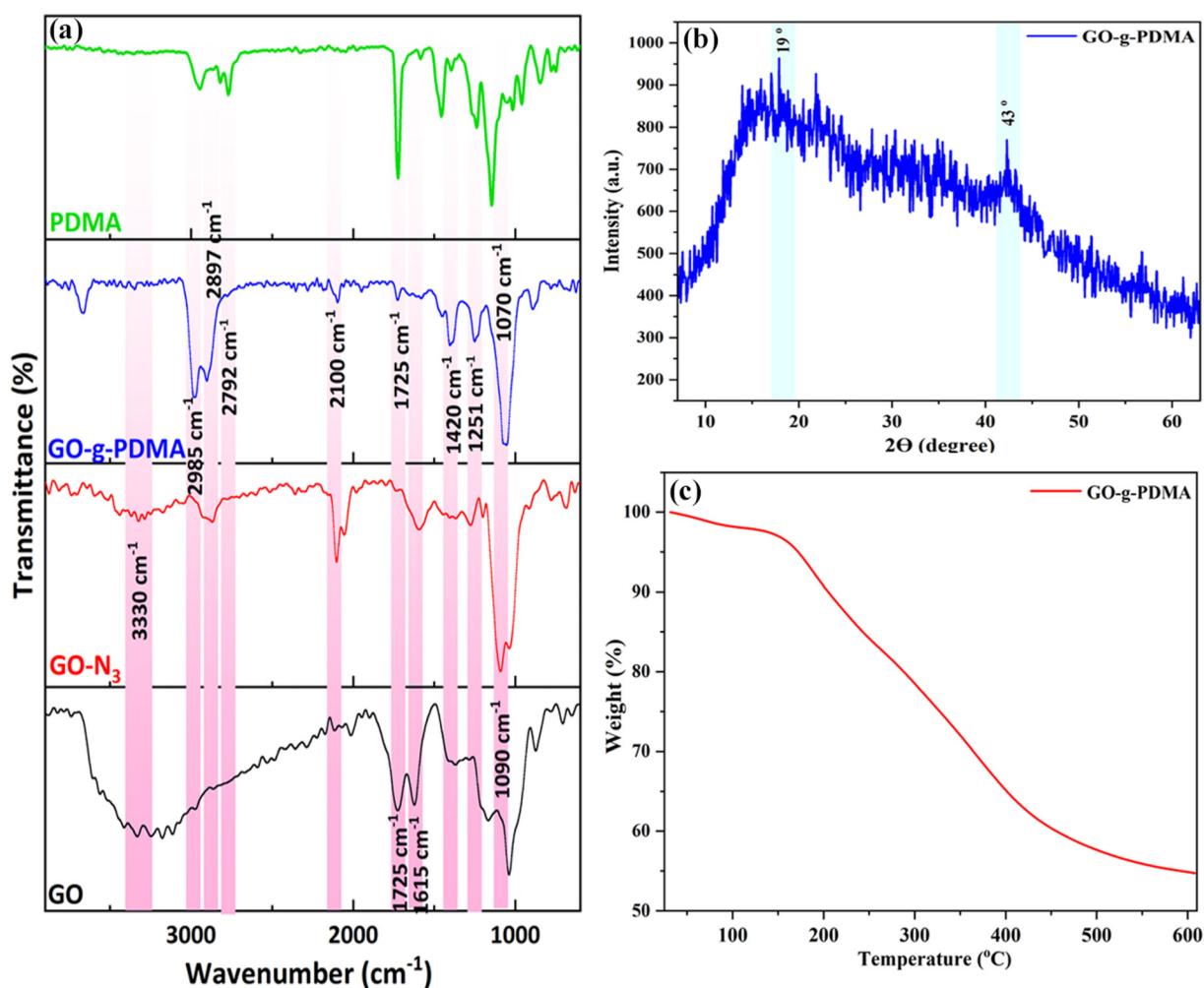
Fig. 3 (a) Comparison of FTIR spectra of the GO, GO-N 3 , GO-g-PDMA, and PDMA polymer, (b) XRD pattern, and (c) TGA curve of the GO-g-PDMA.
