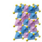
CuFeS 2 - chalcopyrite
