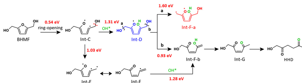
Scheme 2 Reaction mechanism of HHD formation from BHMF, starting with the ring-opening of BHMF (Path 1).
