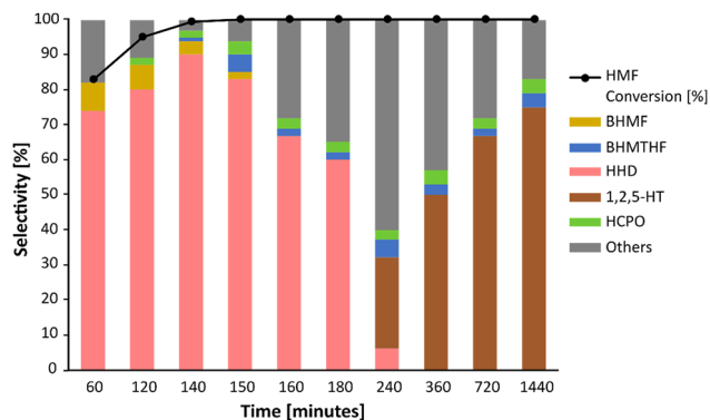
Fig. 1 Influence of reaction time on the product distribution for the HMF hydrodeoxygenation in water over Ru/TiO 2 . Reaction conditions: 0.15 g catalyst, 1 g HMF, 30 mL of water, 70 bar H 2 , 120 °C.
