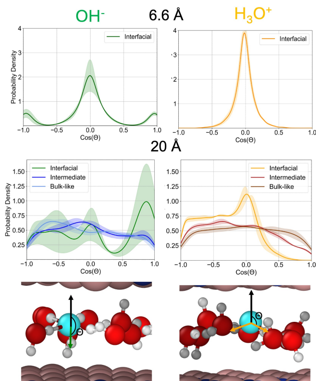
Fig. 4 Cos( \theta ) angle of the respective OH bonds for either the hydroxide or hydronium ion with respect to the normal direction of the hBN surface. For 6.6 Å orientations are calculated with respect to the upper hBN surface. For 20 Å orientations are calculated with respect to either the upper or lower hBN surface depending on if the ion is located below or above the midpoint of the system. The definition of the angle \theta is shown on the respective hydronium and hydroxide snapshots.
