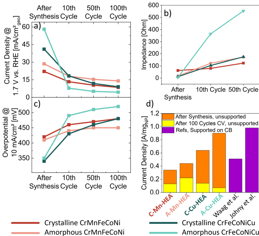
Fig. 6 OER activity of amorphous/crystalline CrMnFeCoNi and CrFeCoNiCu HEA NPs, showing extracted current densities at 1.7 V vs. RHE (a) and overpotentials at 10 mA cm 2 geo -2 (c) from linear sweep voltammetry experiments. (b) Impedance of HEA NPs with different states of the nanoparticle surface (after synthesis, after 10 CV cycles, and after 50 cycles) and (d) comparison of OER current densities extracted at 1.7 V vs. RHE: crystalline and amorphous Mn-containing HEA NPs (C-Mn-HEA and A-Mn-HEA) compared to crystalline and amorphous Cu-containing HEA NPs (C-Cu-HEA and A-Cu-HEA) as well as reference values of CB-supported HEA NPs, reported by Waag et al. 39 (crystalline CrMnFeCoNi HEA NPs obtained via ps-LAL in ethanol) and Johny et al. 41 (amorphous CrMnFeCoNi HEA NPs obtained via ns-LAL in acetonitrile).
