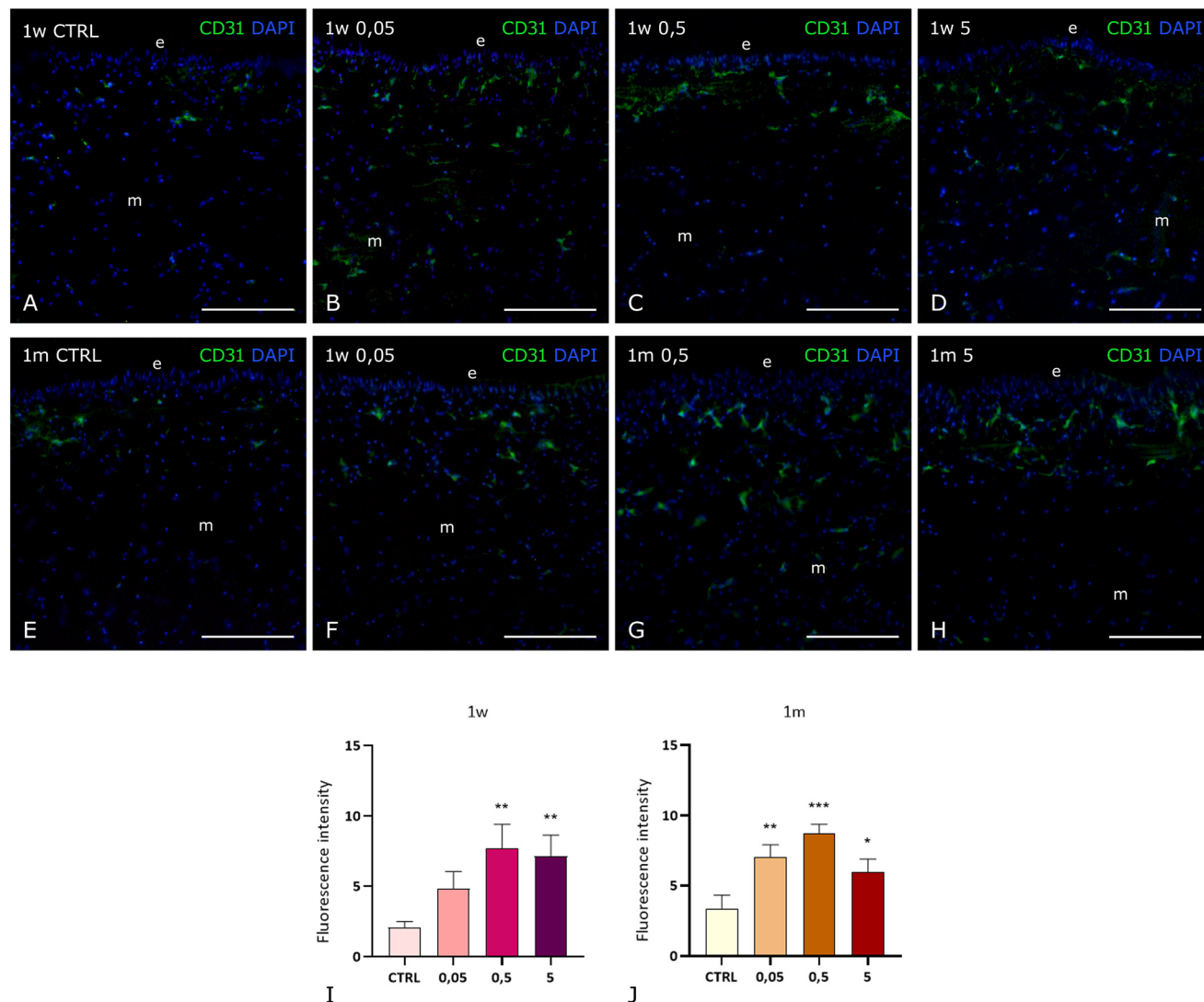
Fig. 5 Chronic exposure to PET NPs sustains CD31 expression and endothelial activation in H. verbaana . Immunofluorescence images of the leech body wall stained with anti-CD31 antibody after 1 week (A–D) and 1 month (E–H) of exposure to PET NPs at 0.05, 0.5, and 5 mg L -1 . In untreated controls (A and E), a weak CD31 signal is detected, indicating minimal vascular presence. Treated animals show a clear, dose-dependent increase in CD31 + endothelial cells at both time points (B–D and F–H). Graphs (I and J) show quantification of CD31 fluorescence intensity, confirming a statistically significant increase after 1 week at all concentrations and after 1 month at 0.5 and 5 mg L -1 . In the graphs, * means that p < 0.05 ; ** means that p < 0.01 ; *** means that p < 0.001 . e epithelium, m muscle, in blue are nuclei stained with DAPI. Bars in A–H: 100 μm.
