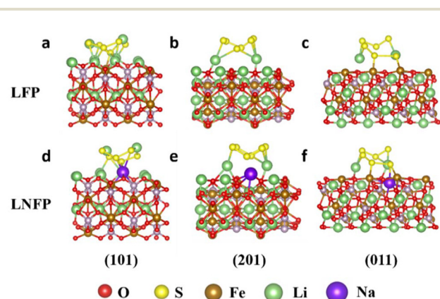
Fig. 1 Theoretical calculations of the adsorption energies of LNFP and LFP for \text{Li}_2\text{S}_6 , key: (a) E_{\text{ads}} = -2.4 \text{ eV} , (b) E_{\text{ads}} = -2.8 \text{ eV} , (c) E_{\text{ads}} = -0.2 \text{ eV} , (d) E_{\text{ads}} = -4.0 \text{ eV} , (e) E_{\text{ads}} = -4.3 \text{ eV} , and (f) E_{\text{ads}} = -2.1 \text{ eV} .
