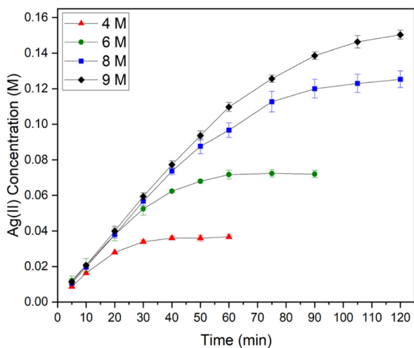
Fig. 3 Ag(II) formation as a function of \text{HNO}_3 concentration over time. Conditions: initial \text{AgNO}_3 stock = 0.5 M \text{AgNO}_3 in variable \text{HNO}_3 concentration, catholyte solution = 8 M \text{HNO}_3 , temperature = 25 °C.
